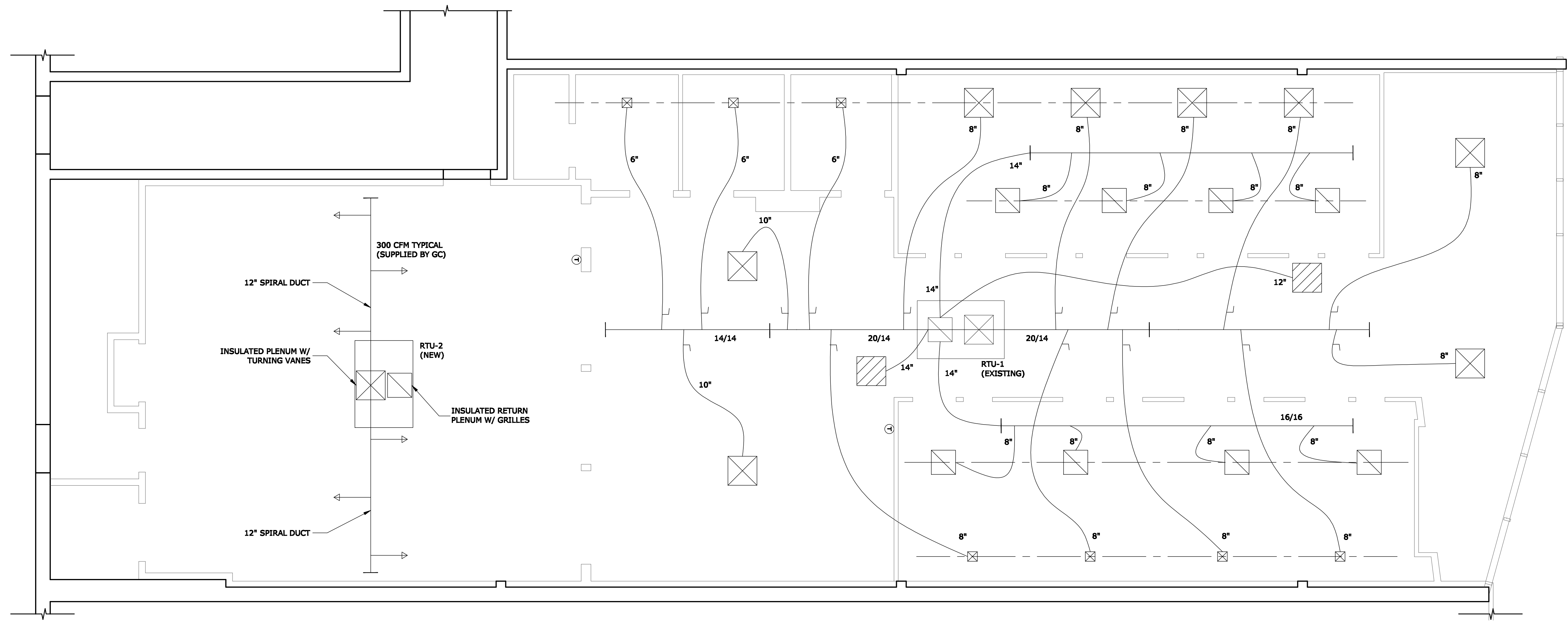
MECHANICAL PLAN 1/4" = 1'-0"
